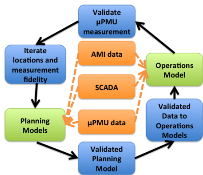
Figure 3. μPMU Workflow
